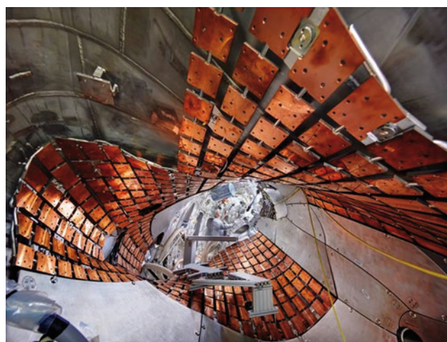
Figure 13. View into the plasma vessel of Wendelstein 7-X. The copper plates establish the support structure for the vessel protection (courtesy: IPP, Bernhard Ludewig).
